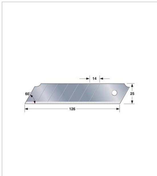
Lame de cutter ROCK HARD BLADE, 25mm
